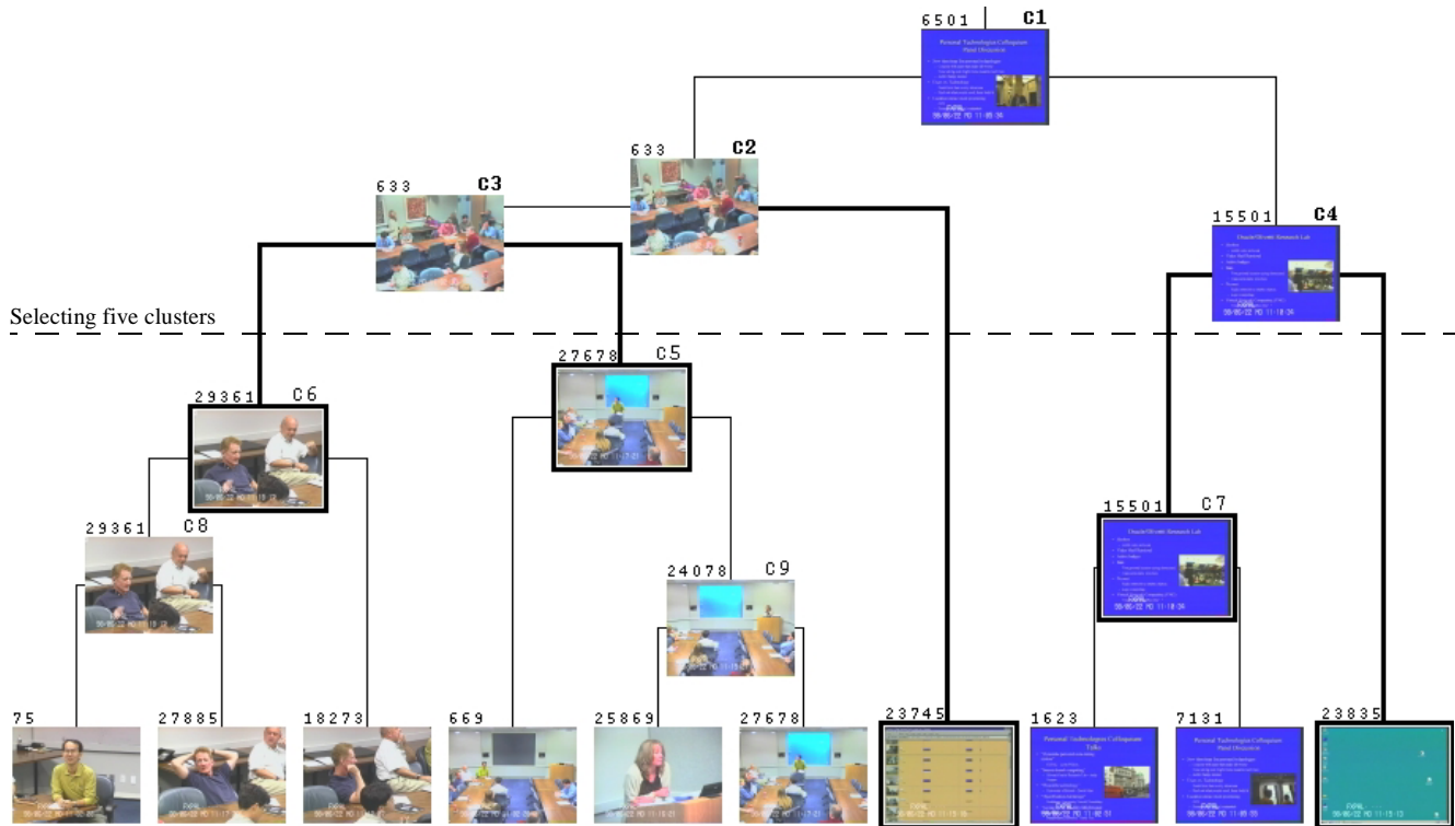
Figure 3. Selecting Five Keyframes from the Cluster Hierarchy
