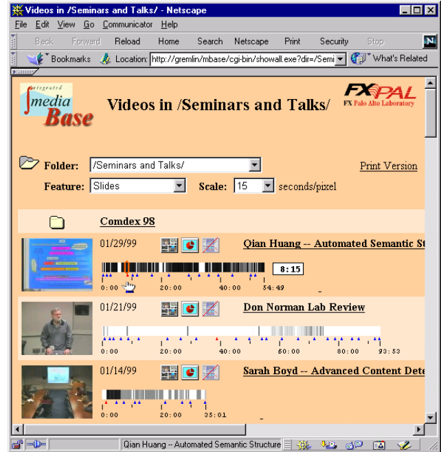
Figure 5. Web-Based Video Directory Browser
