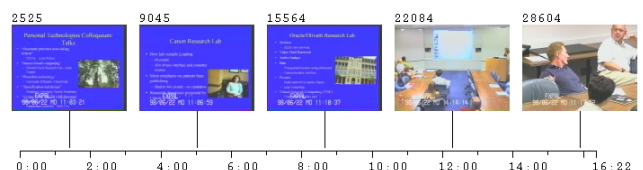
Figure 1. Equidistant Keyframes
