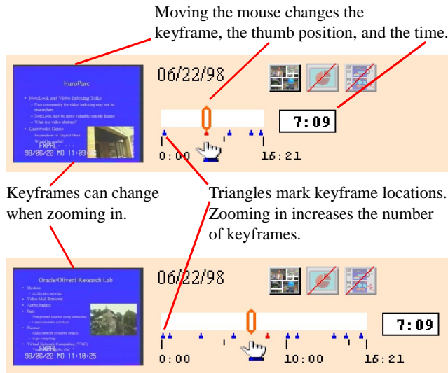
Figure 6. Time Slider for Displaying Keyframes
